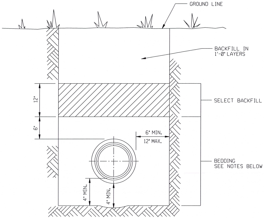
TRENCH CROSS-SECTION
