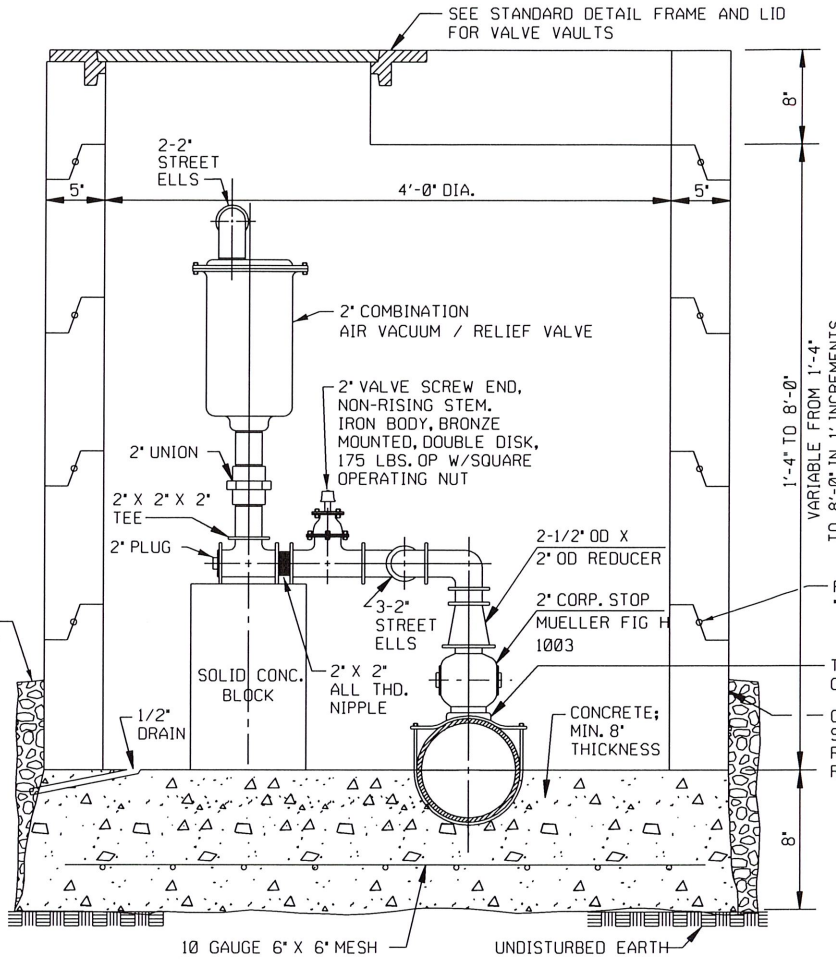
REINFORCED CONCRETE VAULT ALTERNATE FOR STREET TRAFFIC
