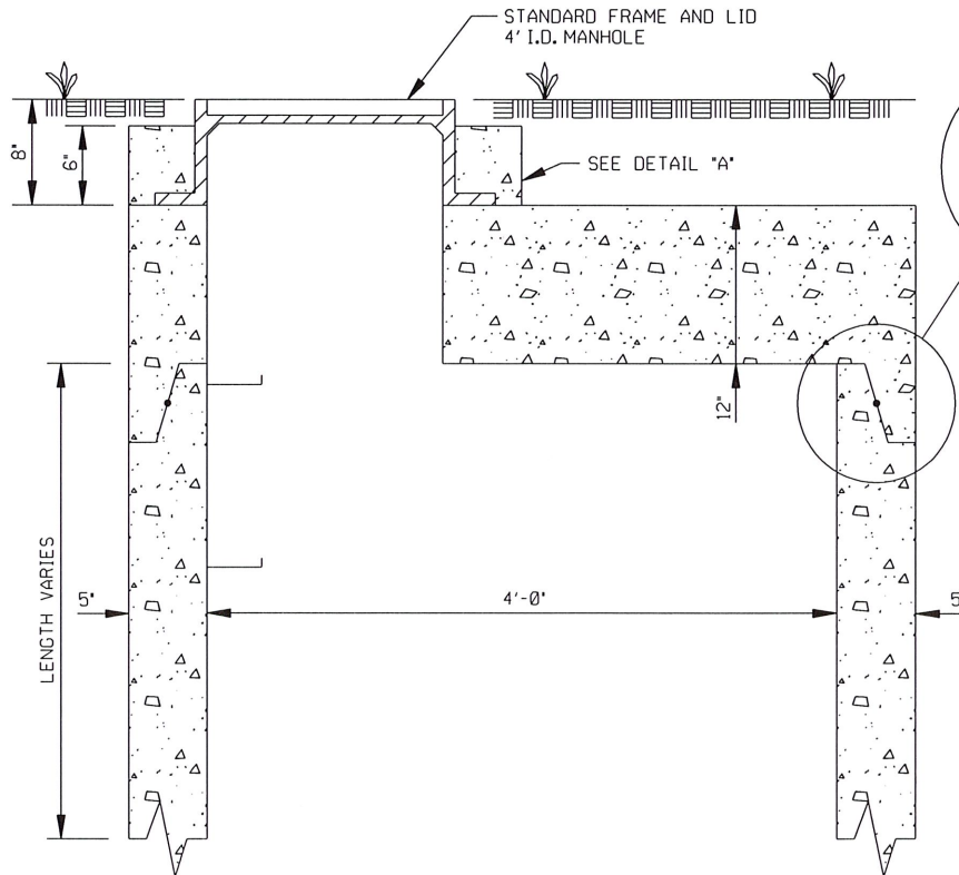
PRECAST MANHOLE IN YARD DETAIL NOT TO SCALE
