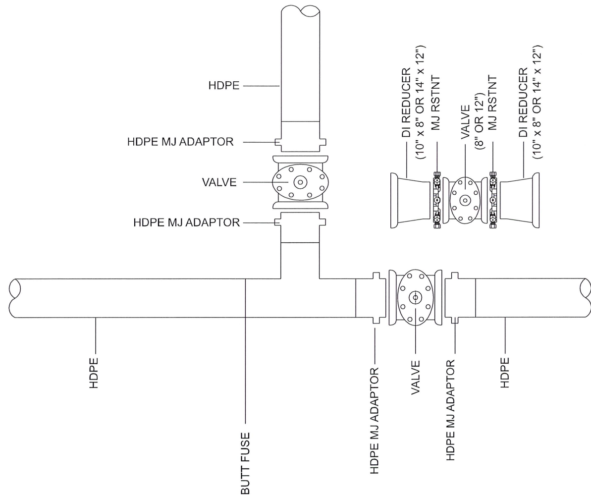
HDPE TEE (HDPE MAIN / HDPE BRANCH)
