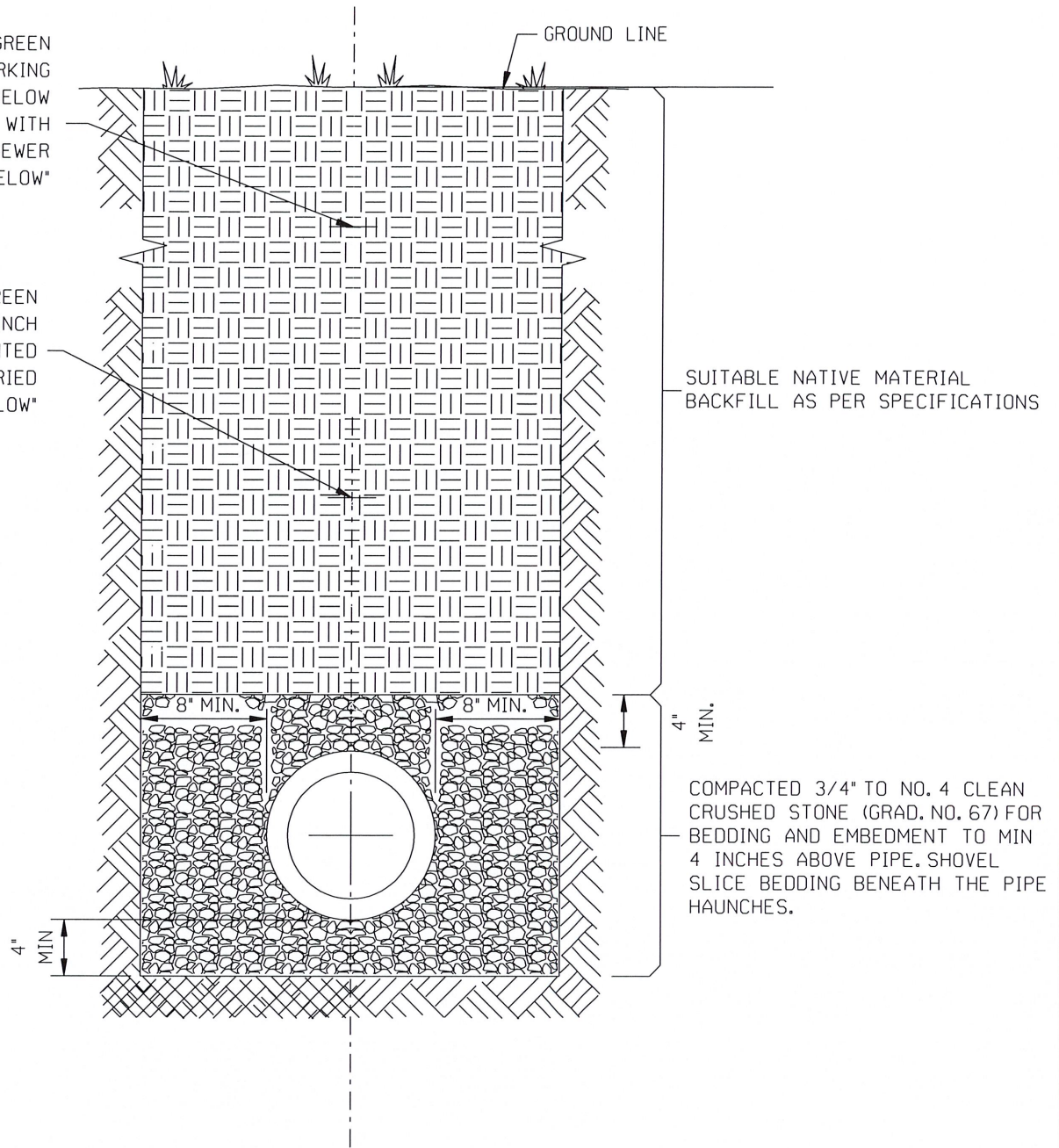
TRENCH CROSS-SECTION FOR DEPTHS UP TO 16' - 0"
