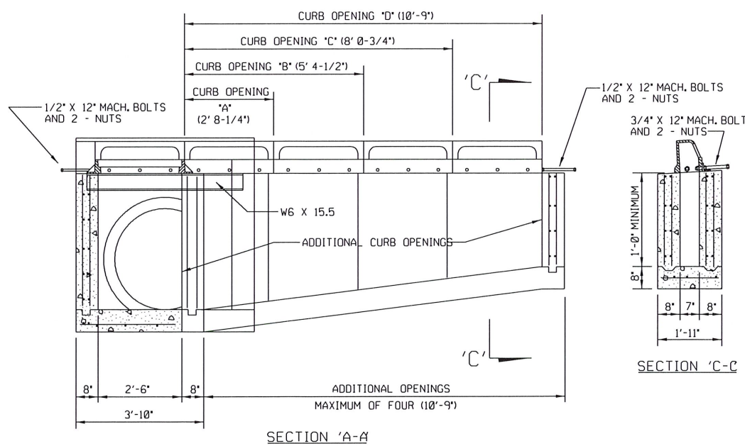
SINGLE GRATE CURB INLET WITH JUNCTION BOX (DESIGN 1-D WITH SMALL JUNCTION BOX SHOWN)
