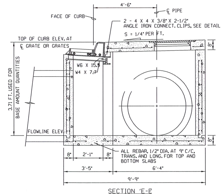
DOUBLE GRATE CURB INLET WITH JUNCTION BOX (DESIGN 2 WITH LARGE JUNCTION BOX SHOWN) 18" THRU 30" LONGITUDINAL PIPE REQUIRES SMALL JUNCTION BOX
