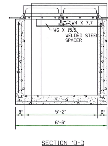
SECTION 'D-D'
