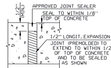
1/2" EXPANSION JOINT
