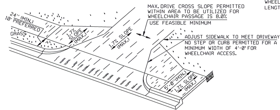
WHEELCHAIR RAMP PROFILES
