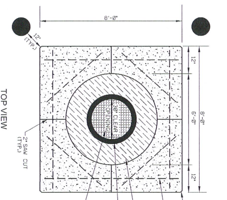
TOP VIEW MANHOLES IN UNPAVED FLOODPLAIN AREAS N.T.S.
